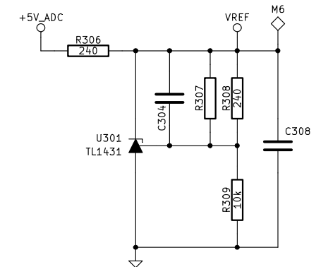
2.56V REFERENCE
