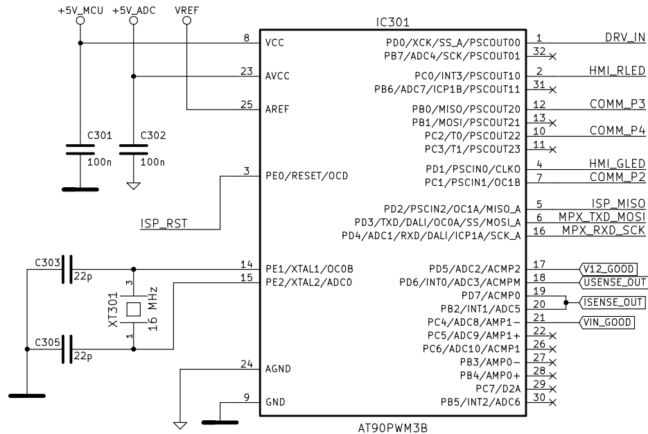
LOW-LEVEL CONTROL LEDS
