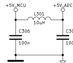
ADC SUPPLY FILTER
