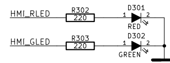
LOW-LEVEL CONTROL LEDS
