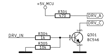
PRIMARY SWITCH INTERFACE DRIVER
